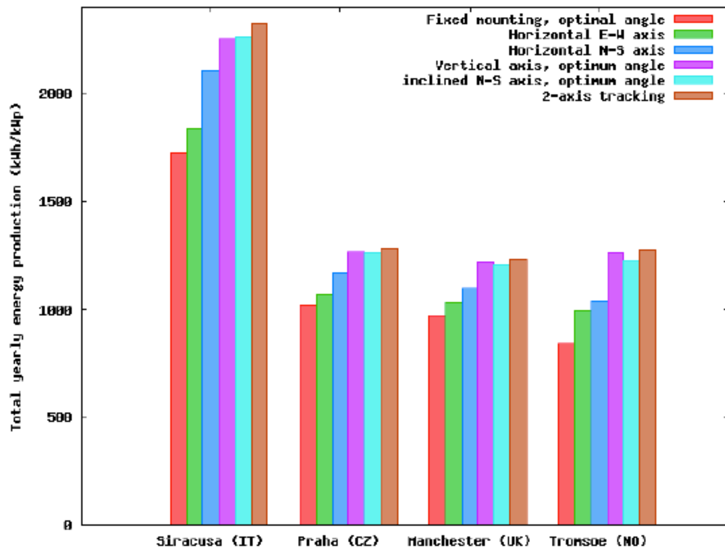
Figure 7: A comparison of the estimated yearly energy output from a 1 kWp PV system (kWh/kWp) using various mounting strategies for four different locations in Europe, representing climate conditions from Mediterranean to Arctic.
